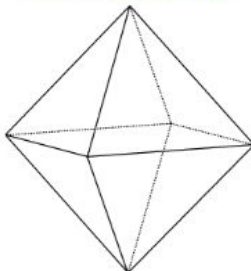
Octahedron
